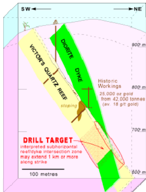
Quartz reef and diorite dyke at Vectors Quartz Mine showing projected down-dip intersection. (Derived from historic mapping in Victorian Government reports.)
